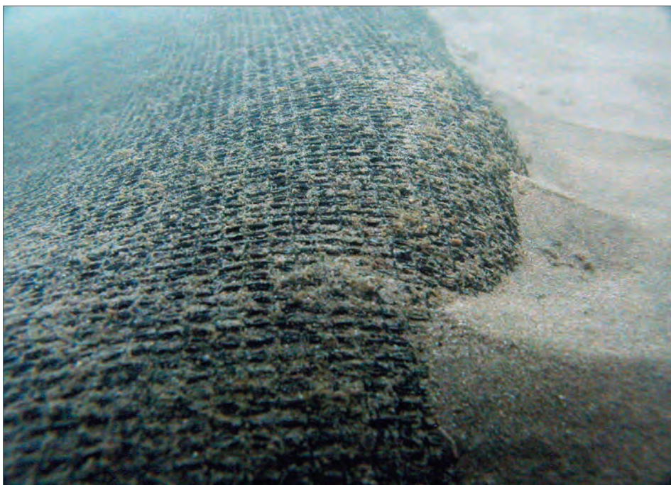
Figure 10.7 A-B First test executed on the Avondster site with shading net (woven, 100 % polypropylene and 60 % density). Old chains served as weights to keep the net down on the seabed.
