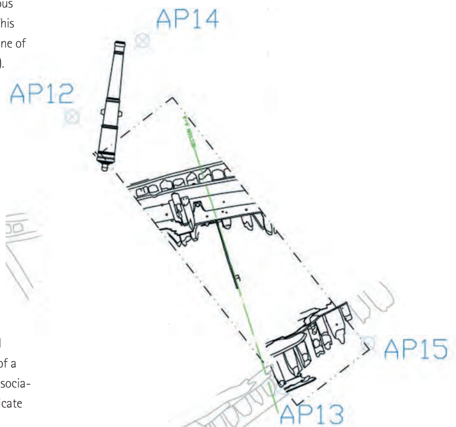
Figure 3.18: The stern trench showing the ship's structure
