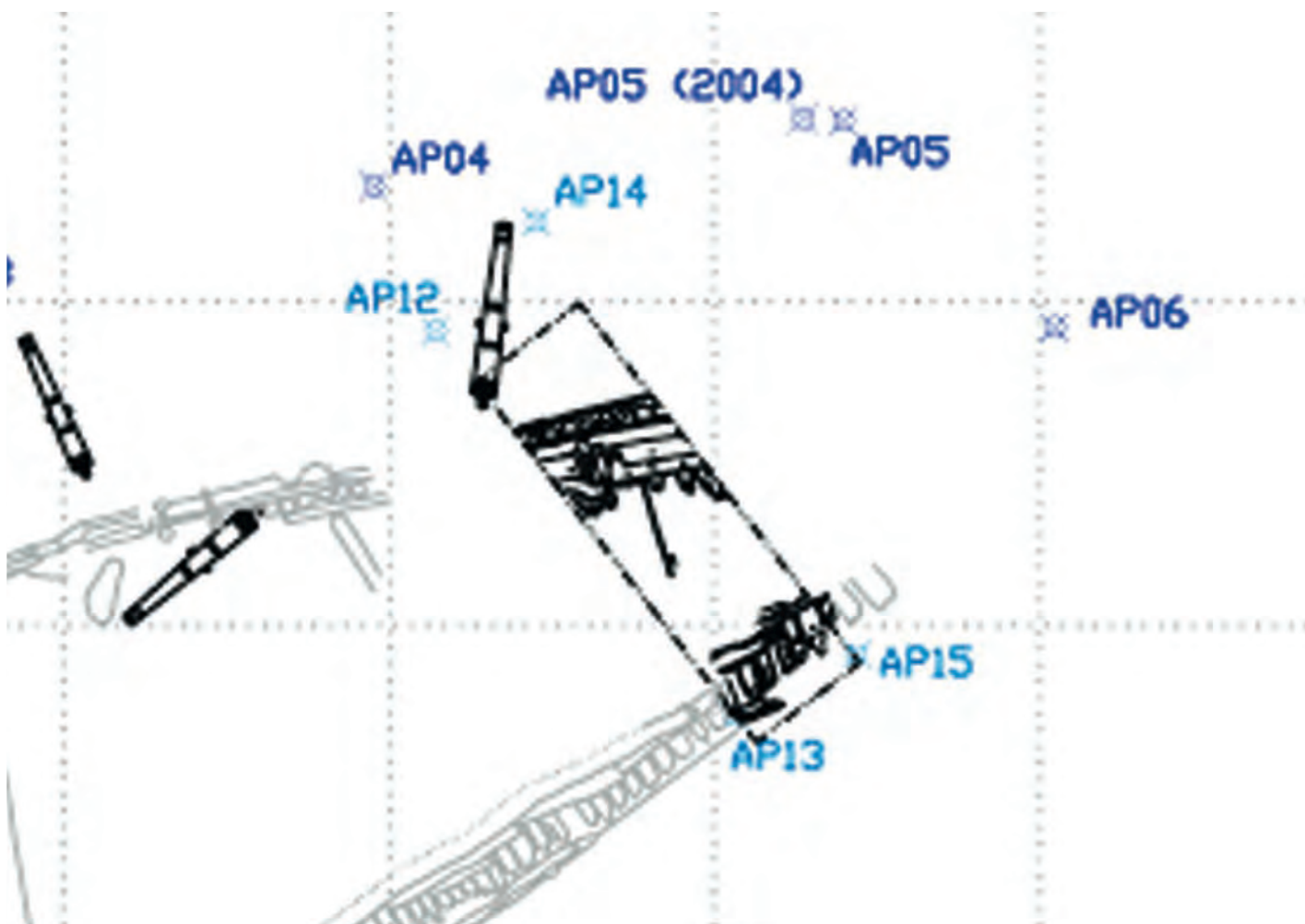
Figure 3.12: Site plan showing location of stern trench
