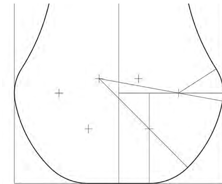
Figure 9.4 Reconstructed midship section of the Avondster based on the Treatise on Shipbuilding from c. 1620–25 (drawing C. Murray).
