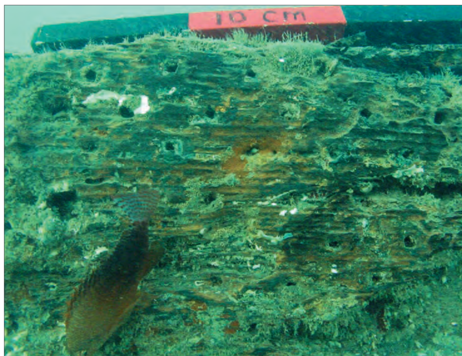
Figure 9.8 Holes left by the iron nails, now corroded away, driven in the external surface of the pine sheathing for extra protection against wood borers.
