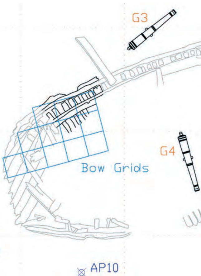
Figure 3.7: Bow timbers in vicinity of excavation grids
