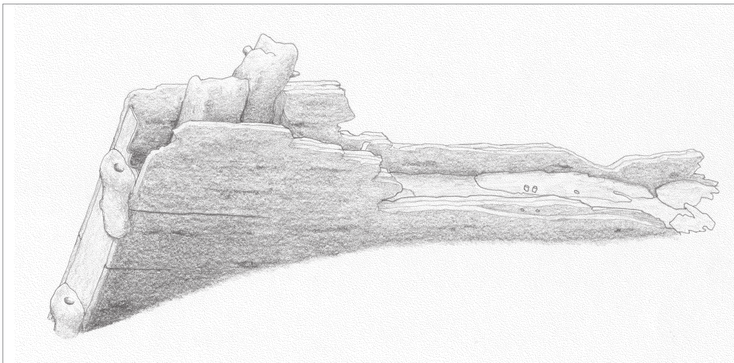
Figure 9.9. Sketch of the lower stern hull section that lies on the seabed detached from the main structure. The sternpost has broken up just above the upper surviving rudder gudgeon (drawing C. Murray).
