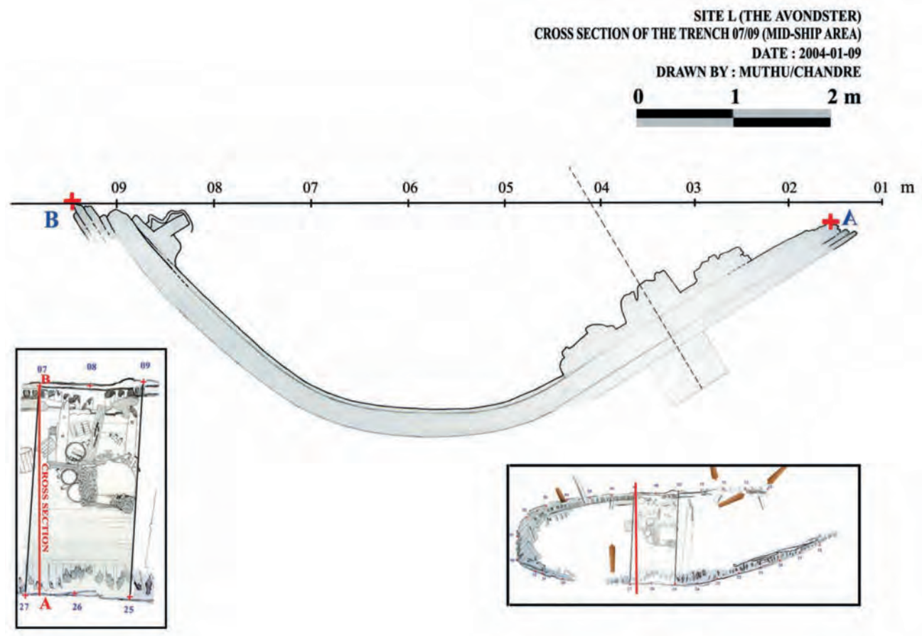
Figure 8.23 Cross section of trench 07/09
