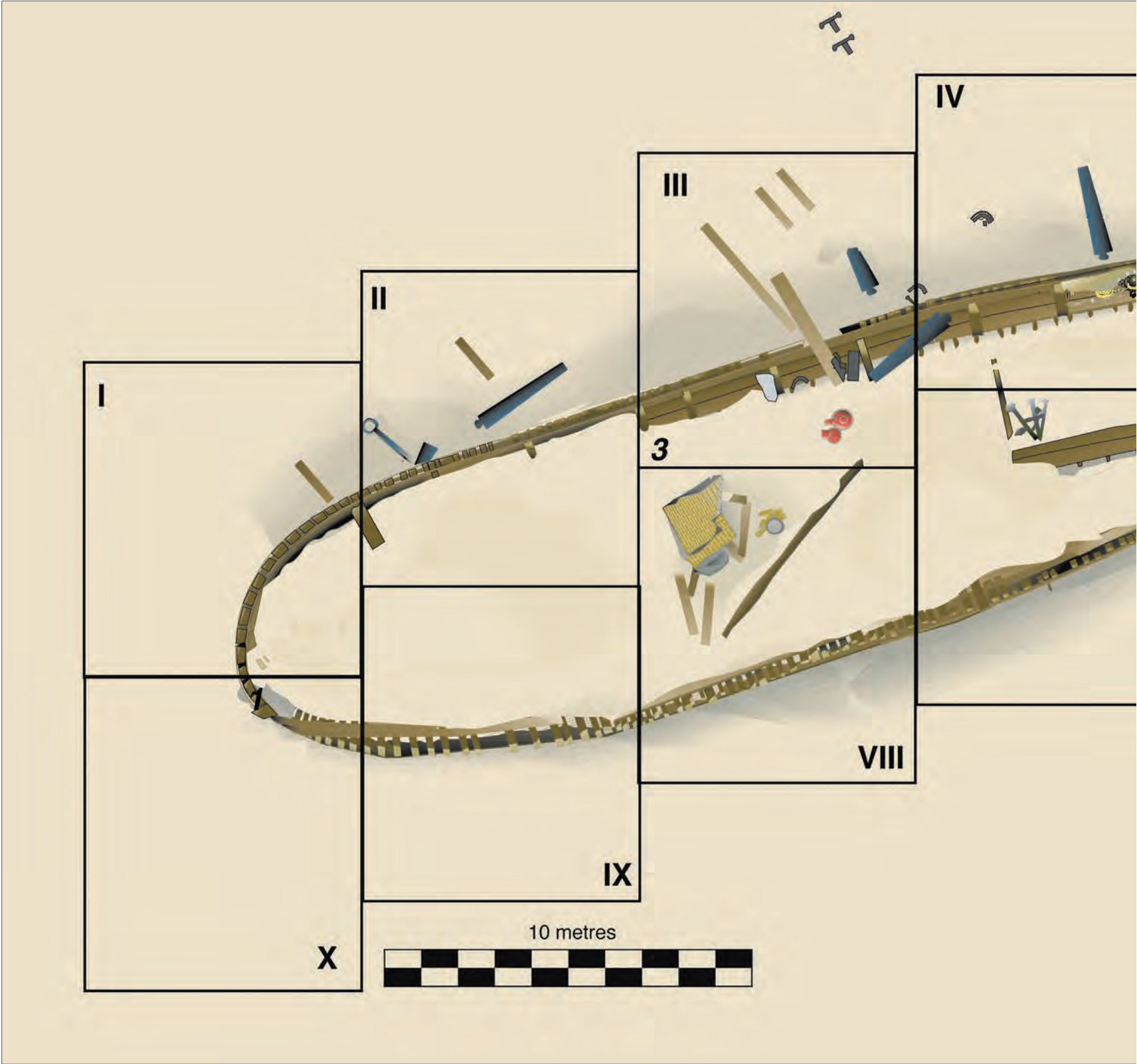
Figure 2.3 Site plan Avondster 1998, drawing R. Parthesius
